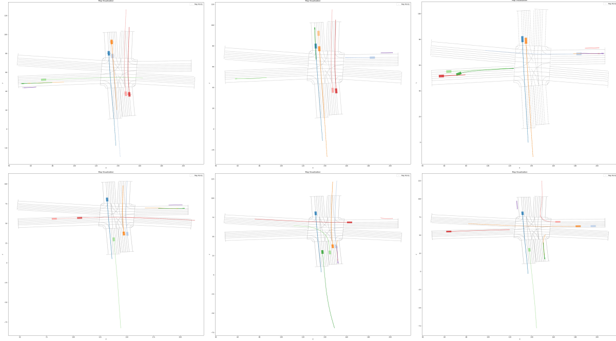
Figure 2. Visualization of six diverse scenarios generated by SimFormer. The blue vehicle denotes the ego agent. Each frame includes five vehicles, two cyclists, and one pedestrian.
