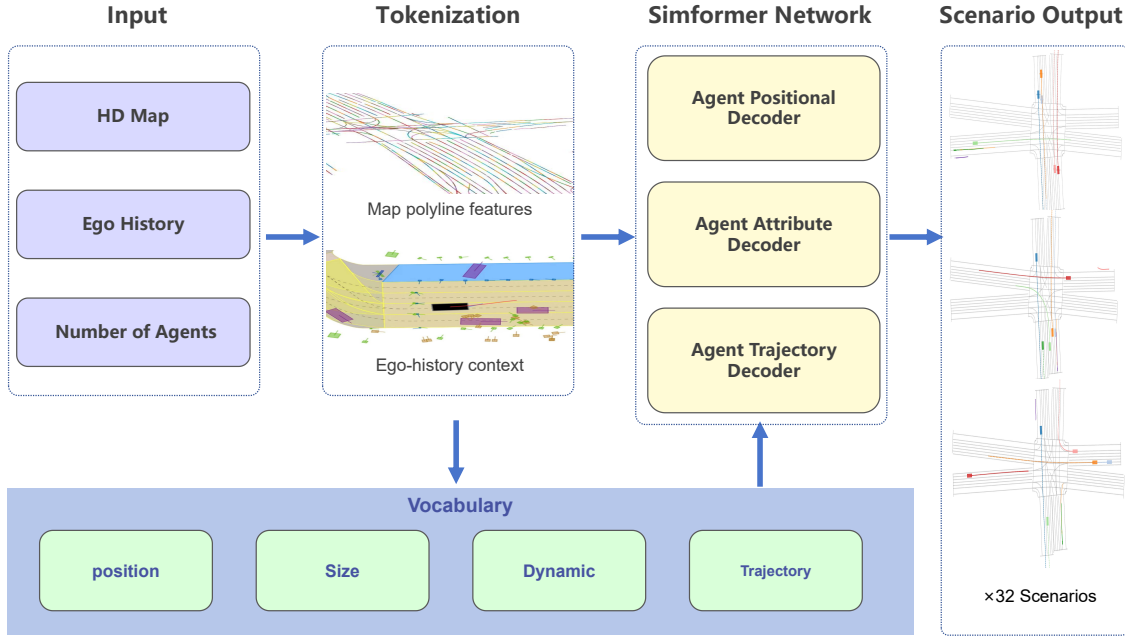
Figure 1. Model Architecture.
